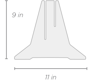
2-Slot Foot
